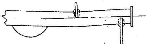
(illus. A) warpage caused by welding on one side of housing.
